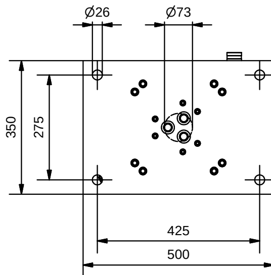
Bottom view (1:10)
